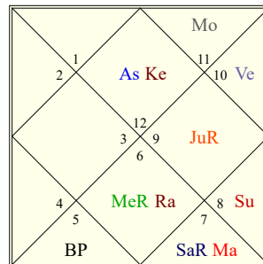
Shodashamsha (conveyances)
