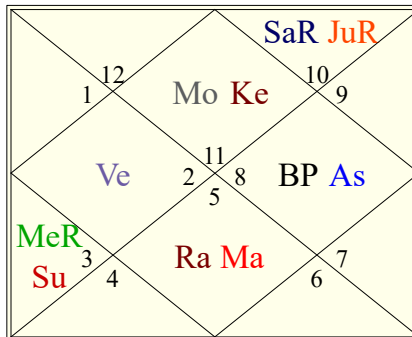
Equal Bhava
