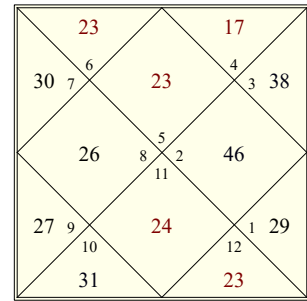
Samudaya Ashtakavarga
