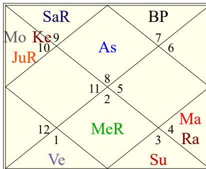
Equal Bhava
