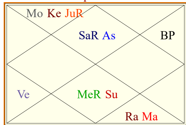
Cuspal Chart
