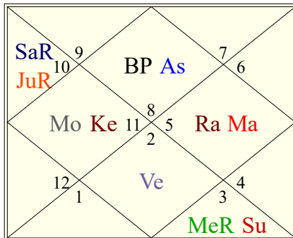
Sripati Bhava
