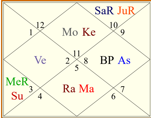
Moon Chart
