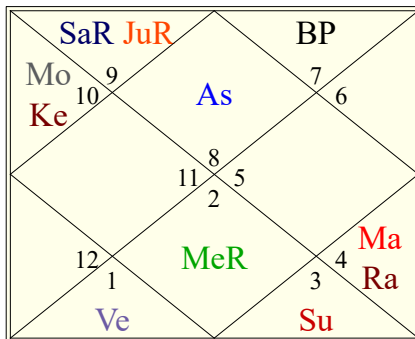
Sripati Bhava
