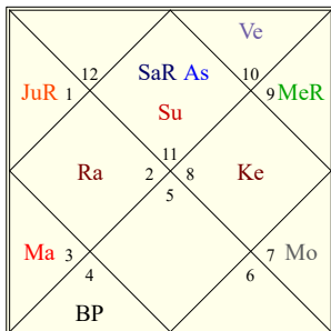
Dwadashamsha (parents)
