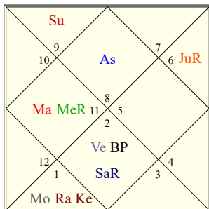
Trimshamsha (misfortunes)
