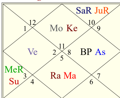
Bhava Lagna
