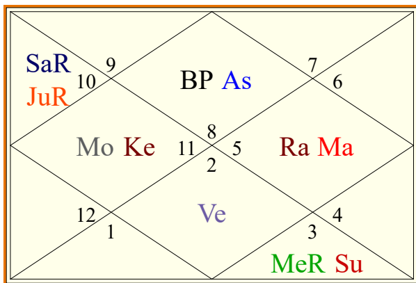
Birth Chart
