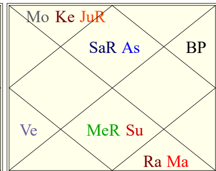
KP Bhava
