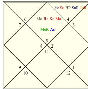
Saptamsha (children)
