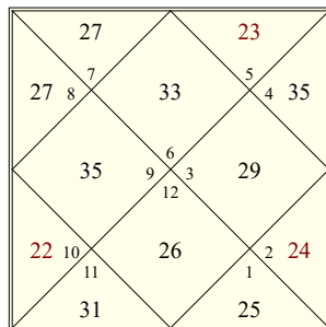
Samudaya Ashtakavarga
