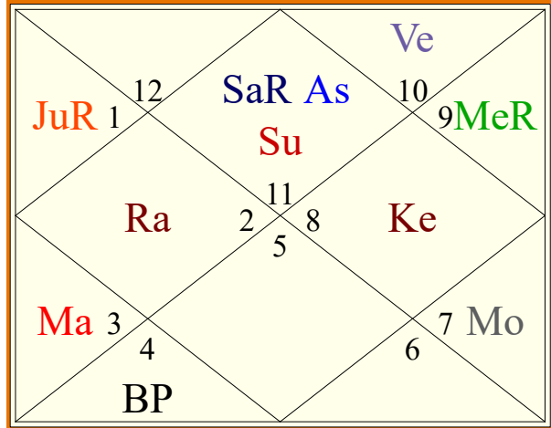
Navamsha
