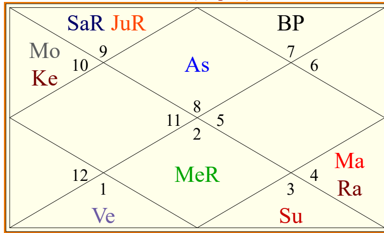
Bhava(Sripati)
