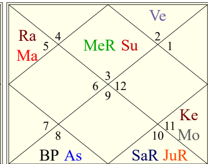
KP Bhava
