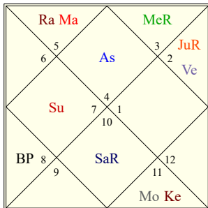
Navamsha (spouse)
